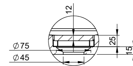
DETAIL AN SCALE 1 : 5
