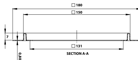
RP15-7 150x150 mm (7 mm hoog)
