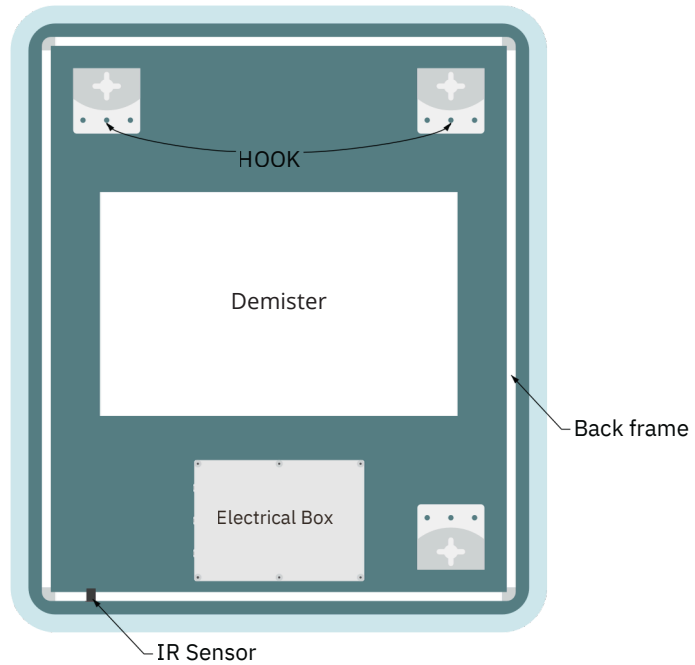
BACK VIEW
