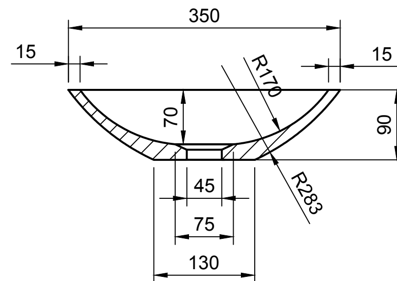
SECTION VIEW B-B
