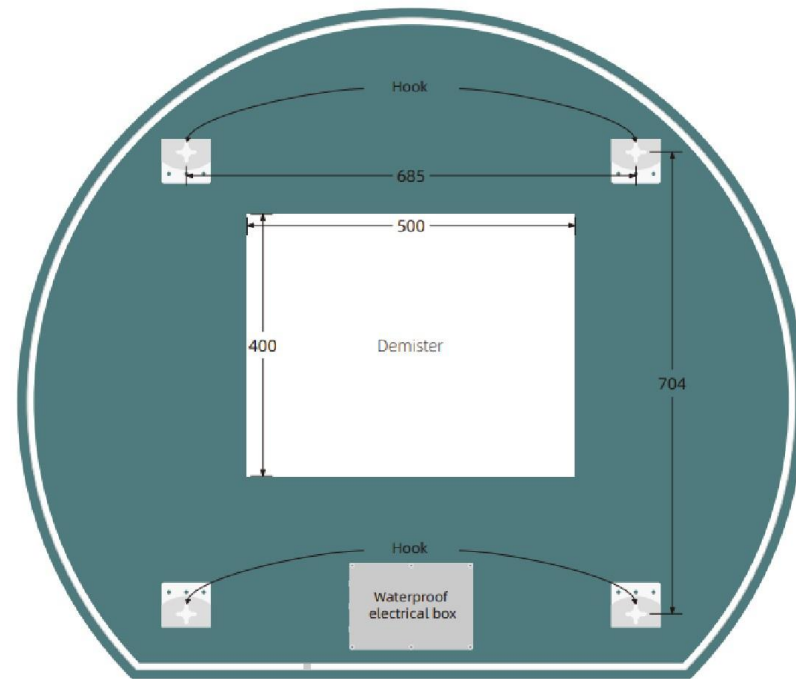
Back view
