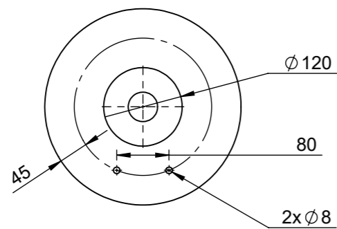
SECTION AF-AF
