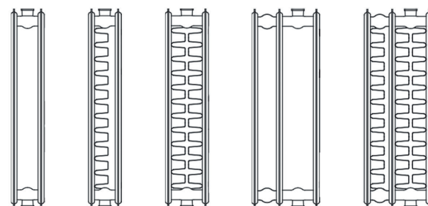
type 20 type 21 type 22 type 30 type 33
