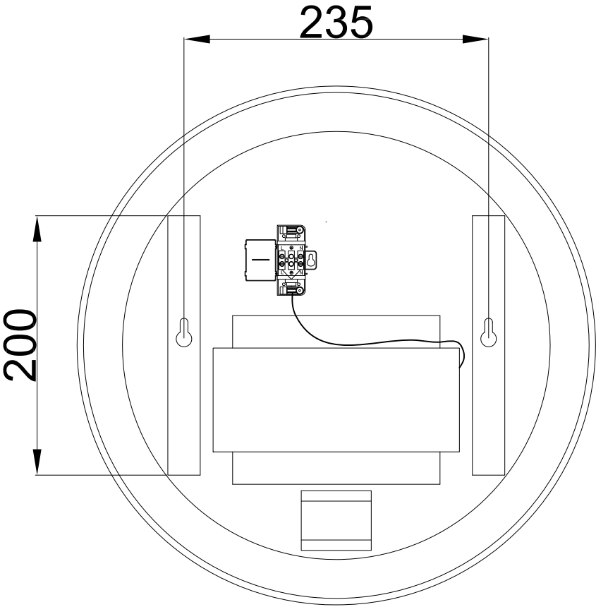
BACK VIEW
