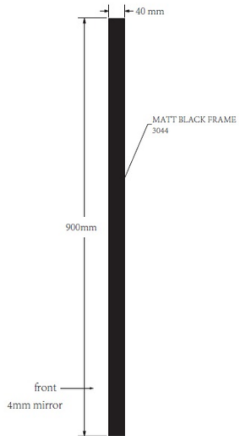
SIDE VIEW
