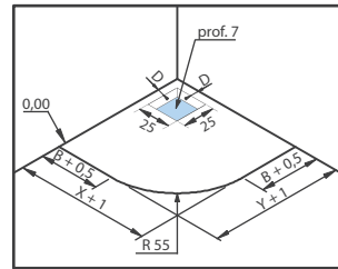
Pre-installation
