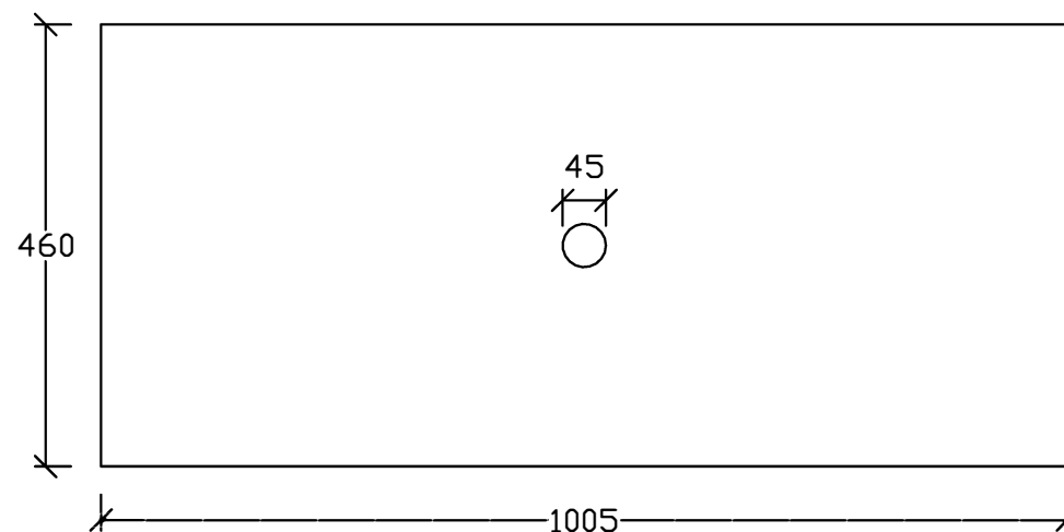
Bottom View
