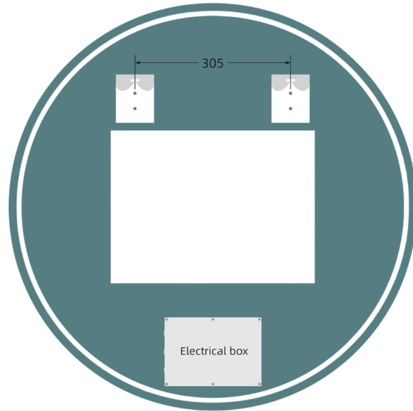
Back View
