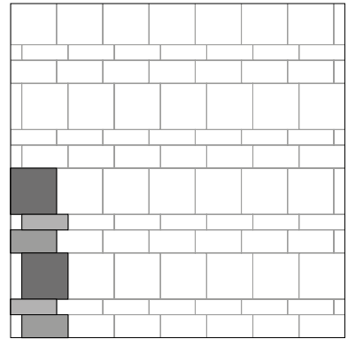
GS-3 18% /m 2 20 x 60 cm / 8 x 24 inch 27% /m 2 30 x 60 cm / 12 x 24 inch 55% /m 2 60 x 60 cm / 24 x 24 inch
