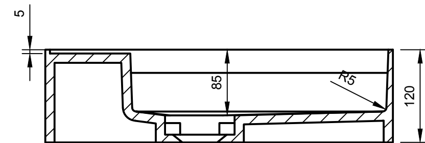
B-B (1:5)
