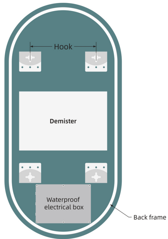
BACK VIEW
