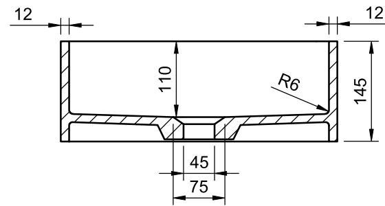
SECTION VIEW B-B
