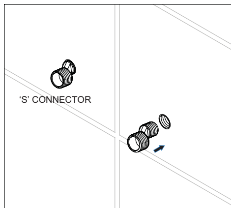
FIG. 2 FITTING THE 'S' CONNECTORS
